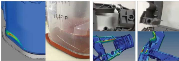
Simulating drop tests with RADIOSS shows the root cause of failure and helps with finding corrective actions
