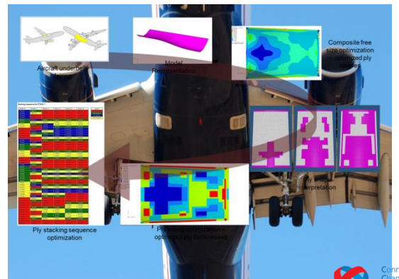
Underbelly Fairing Optimization
